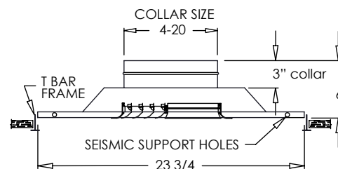
700MA-3in (shown with 3" tall premium round collar)
