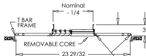
700MA with Standard Square Collar
